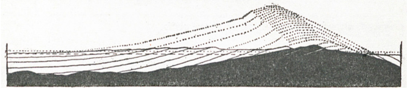
Fig. 60—Ideal section of the uptilted and down-worn half of the same atoll, drawn on twice the scale of Figure 59.
